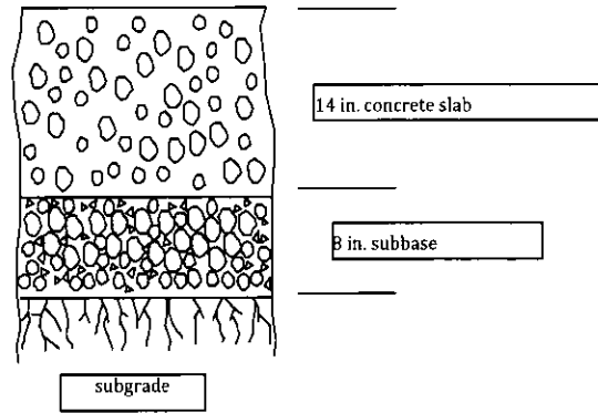
Figure A2-2. Rigid Pavement Example Cross-Section
