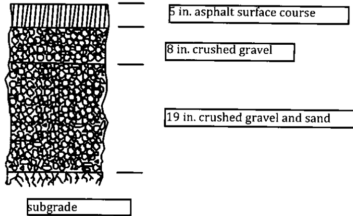
Figure A2-1. Flexible Pavement Example Cross-Section
